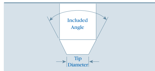
Figure 1: Truncated cone electrode tip profile
